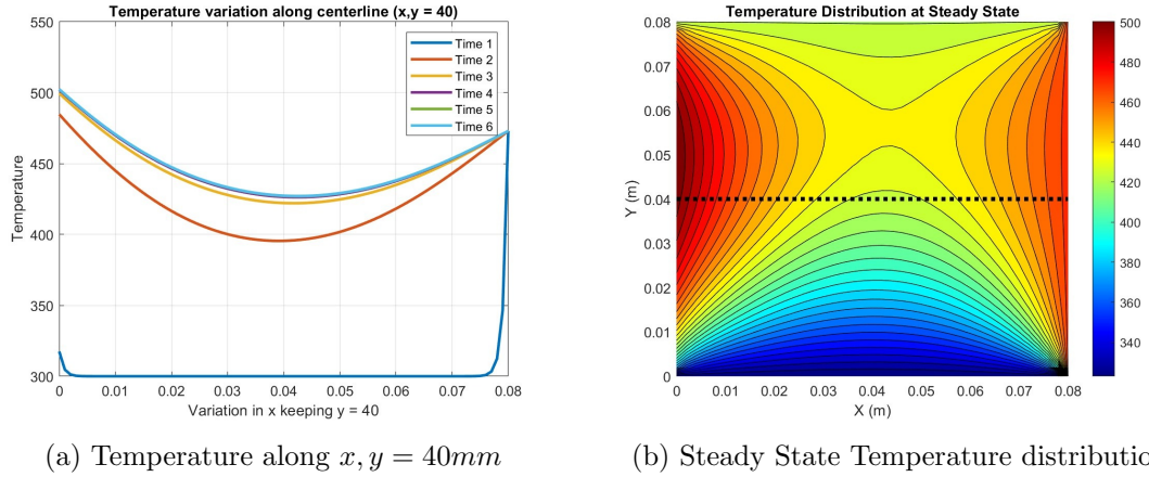
Figure 8: Temperature variation along the centre lines ( x, y = 40\text{mm} ) of the domain.
