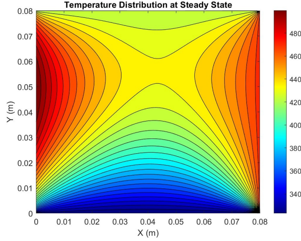
Figure 2: Temperature distribution for N = 81 grid points using the explicit scheme
