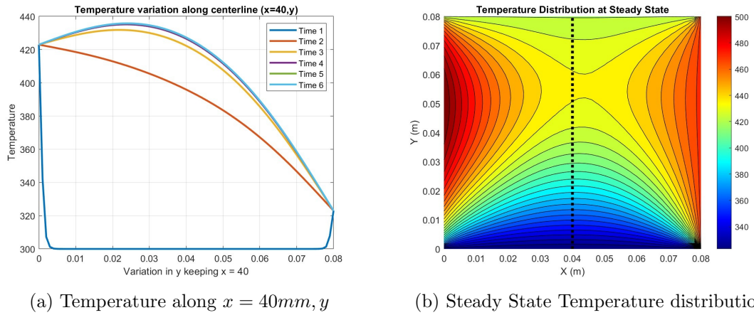
Figure 10: Temperature variation along the centre lines ( x = 40\text{mm}, y ) of the domain.
