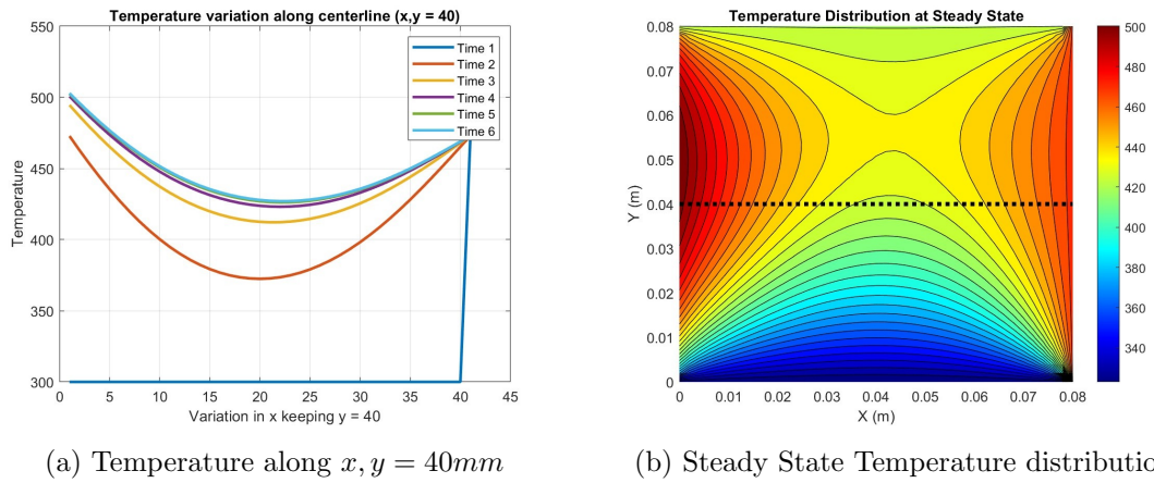
Figure 5: Temperature variation along the centre lines ( x, y = 40\text{mm} ) of the domain.
