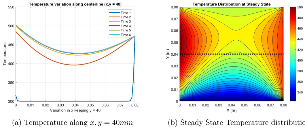
Figure 11: Temperature variation along the centre lines ( x, y = 40\text{mm} ) of the domain.
